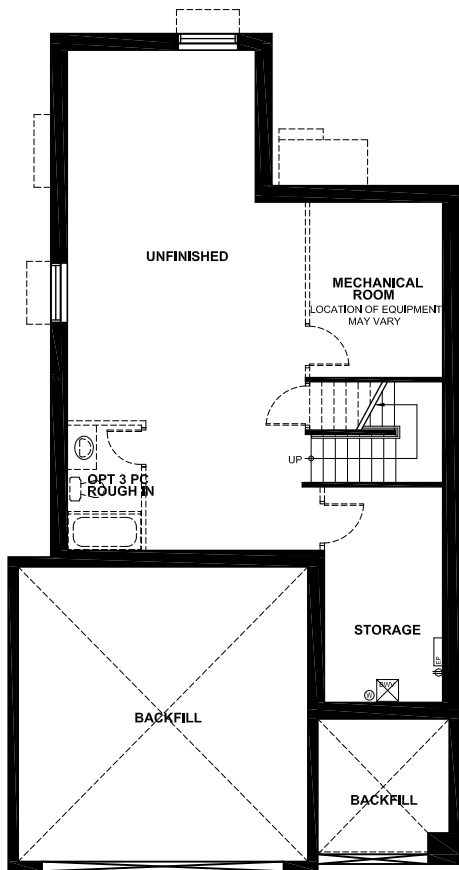
UNFINISHED BASEMENT PLAN
