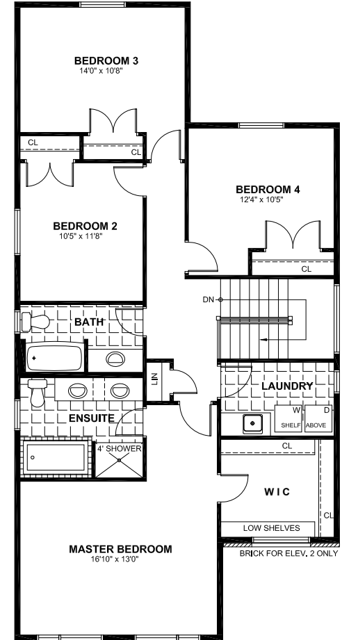
SECOND FLOOR PLAN W/ OPTIONAL 4 PC ENSUITE
