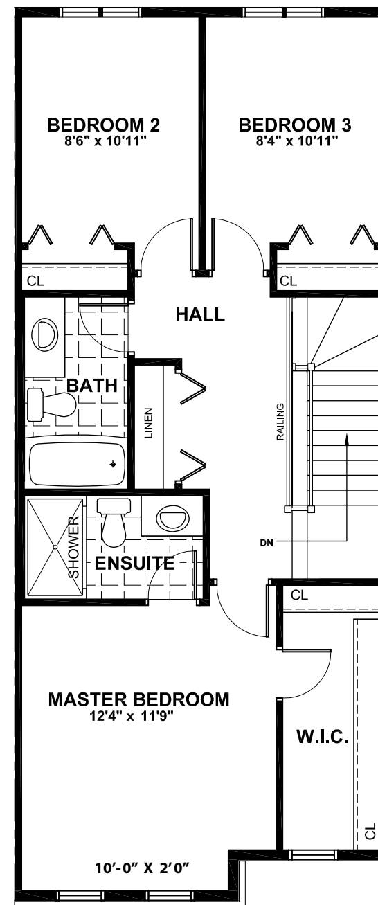
SECOND FLOOR PLAN OPTIONAL ENSUITE
