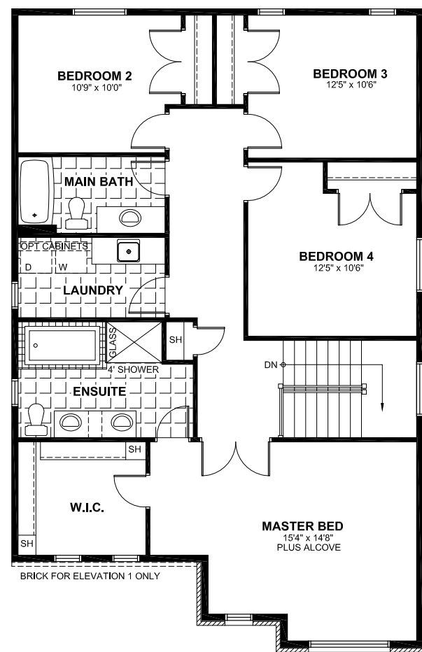
SECOND FLOOR WITH OPTIONAL 4 PIECE ENSUITE
